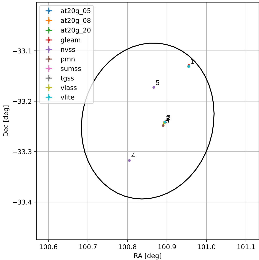
4FGL J0643.4-3314
