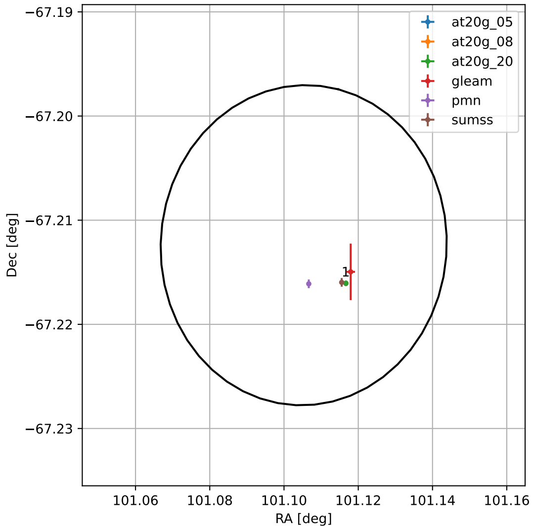
4FGL J0644.4-6712
