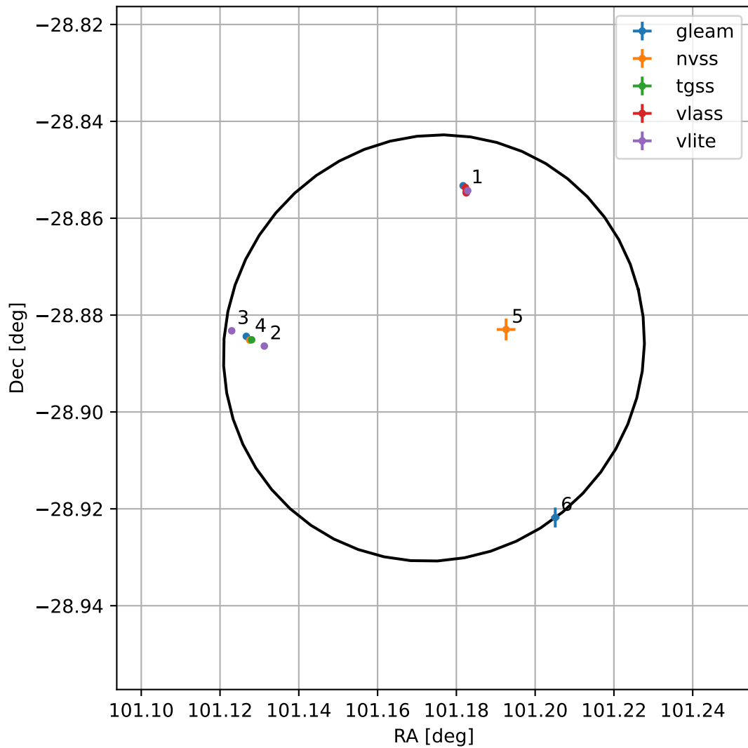
4FGL J0644.6-2853
