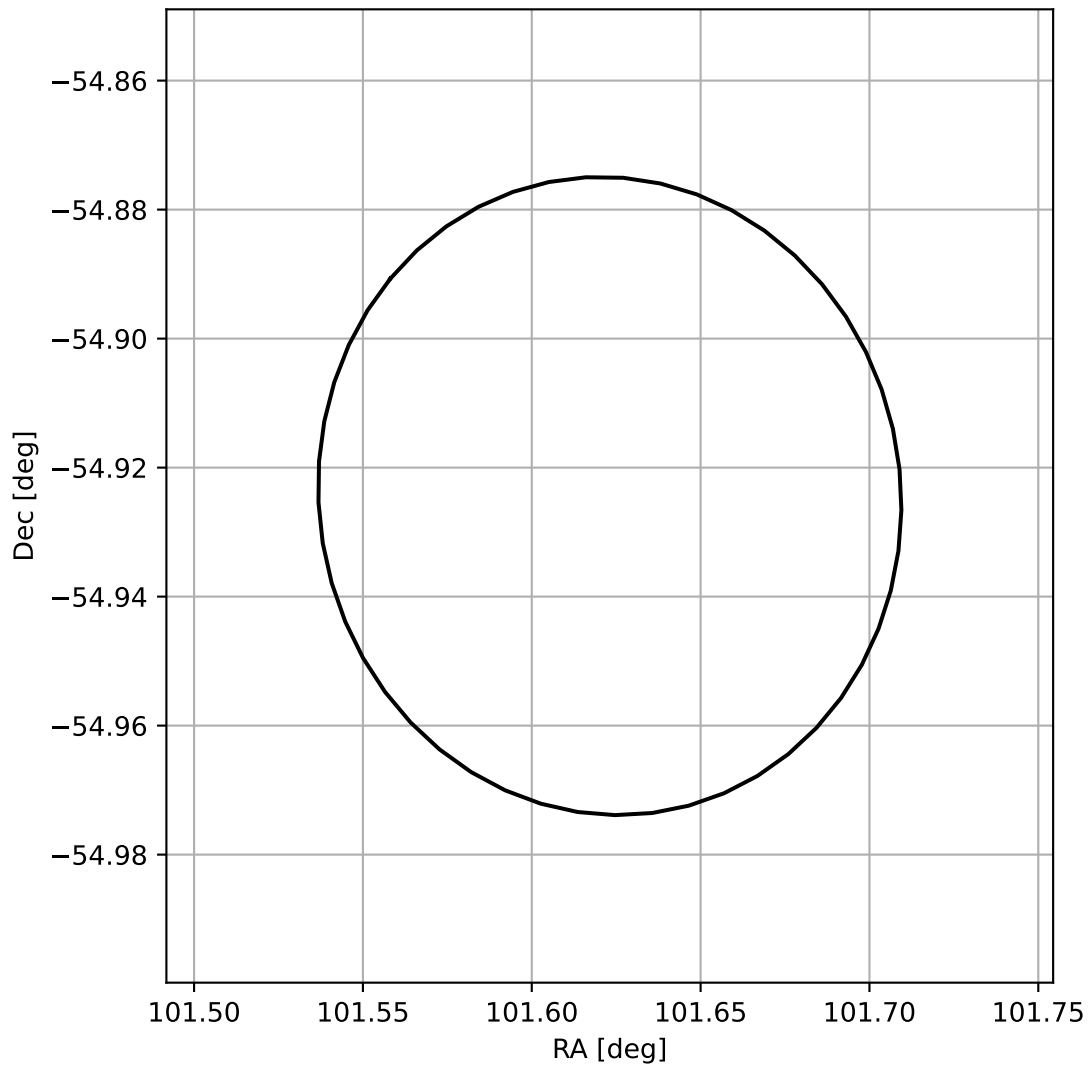
4FGL J0646.4-5455
