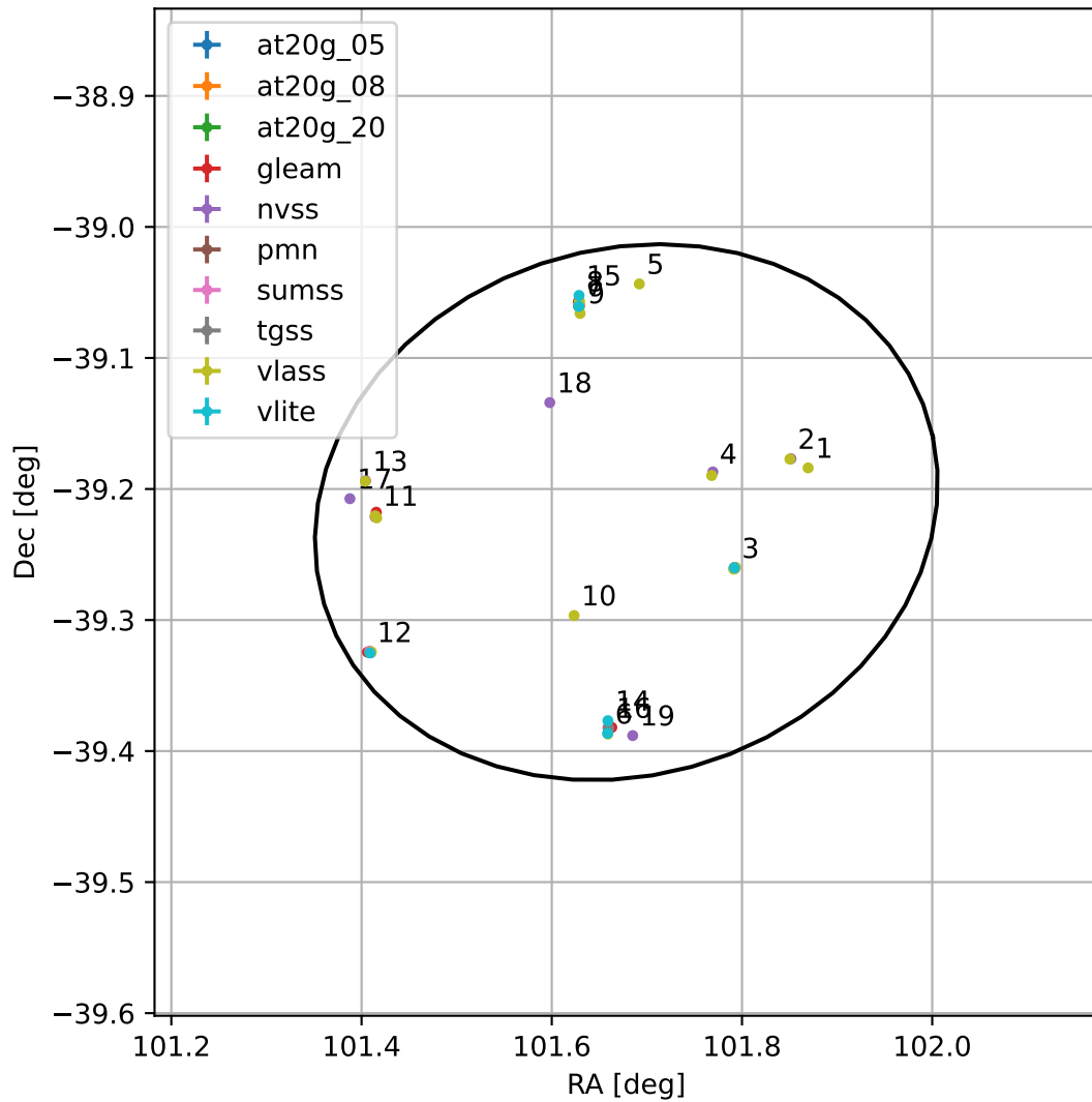
4FGL J0646.7-3913
