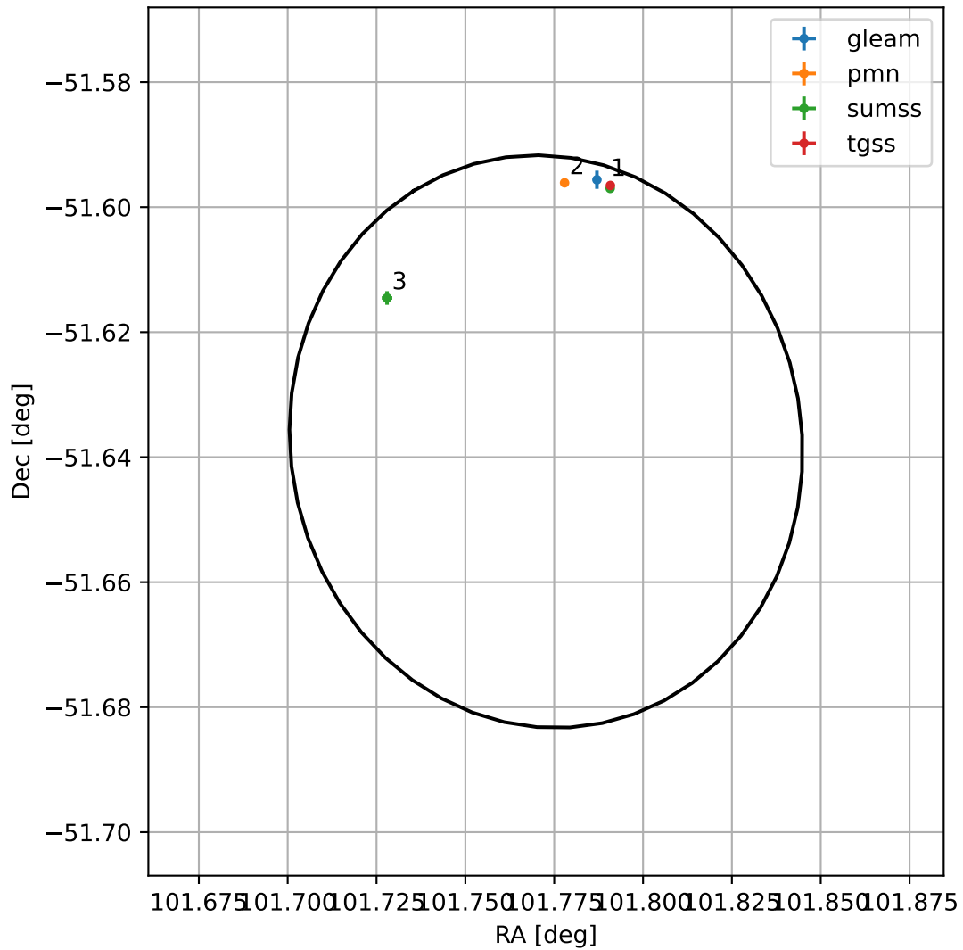
4FGL J0647.0-5138
