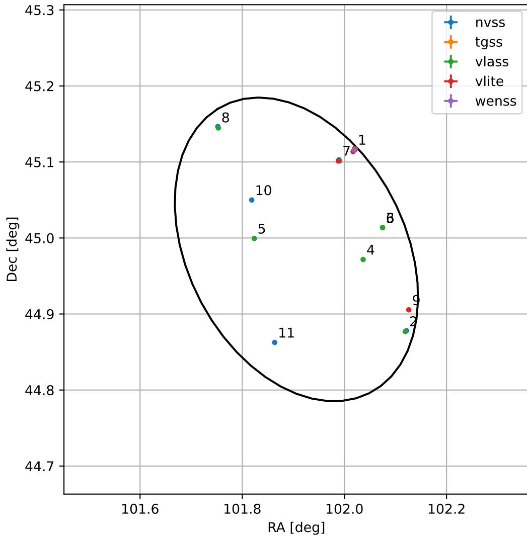
4FGL J0647.6+4459
