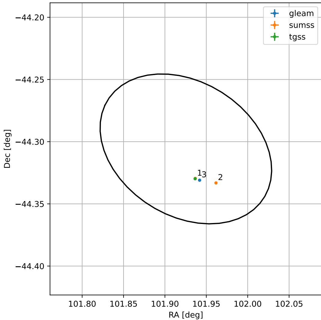
4FGL J0647.7-4418
