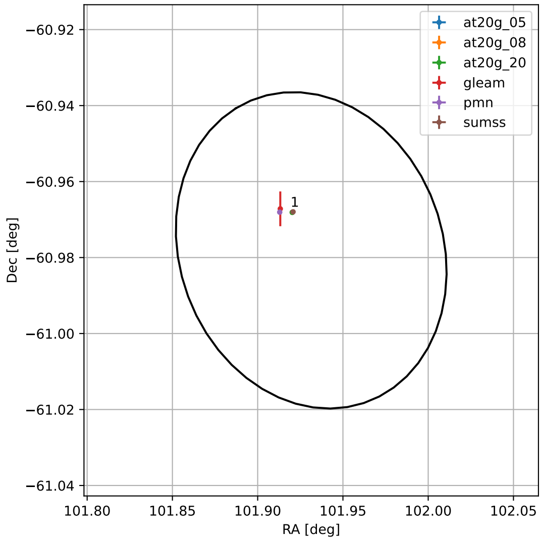
4FGL J0647.7-6058
