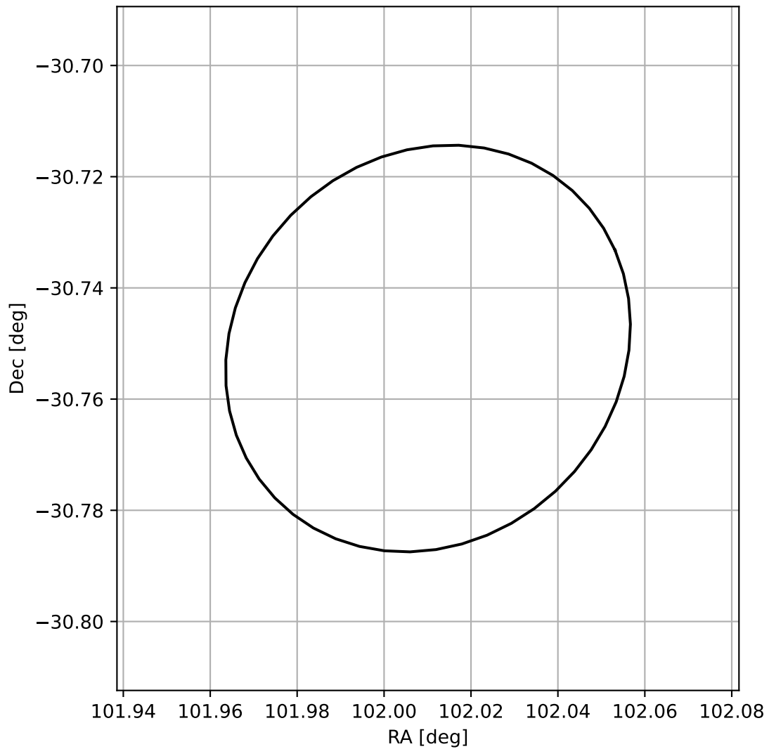
4FGL J0648.0-3045
