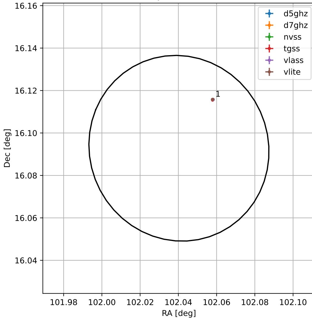
4FGL J0648.1+1605
