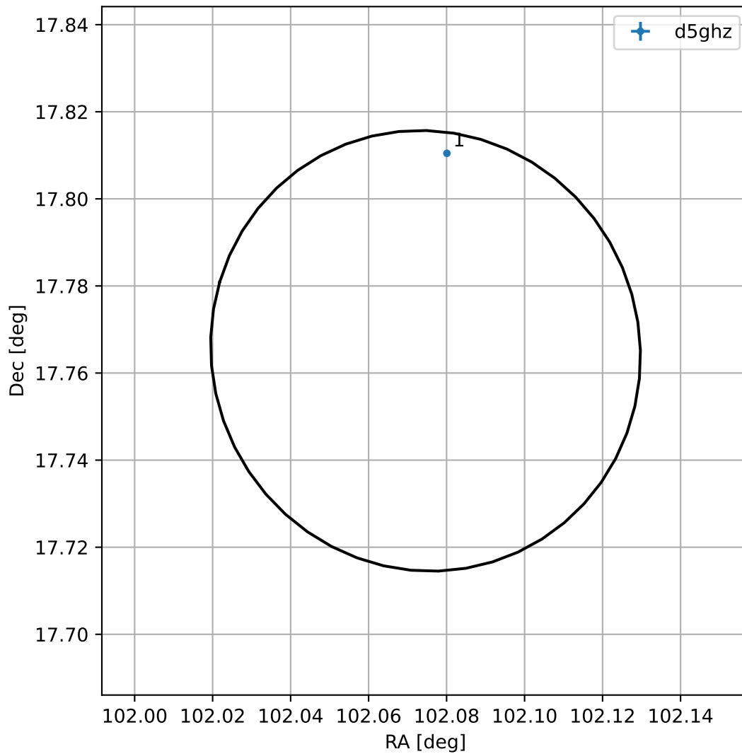
4FGL J0648.2+1745
