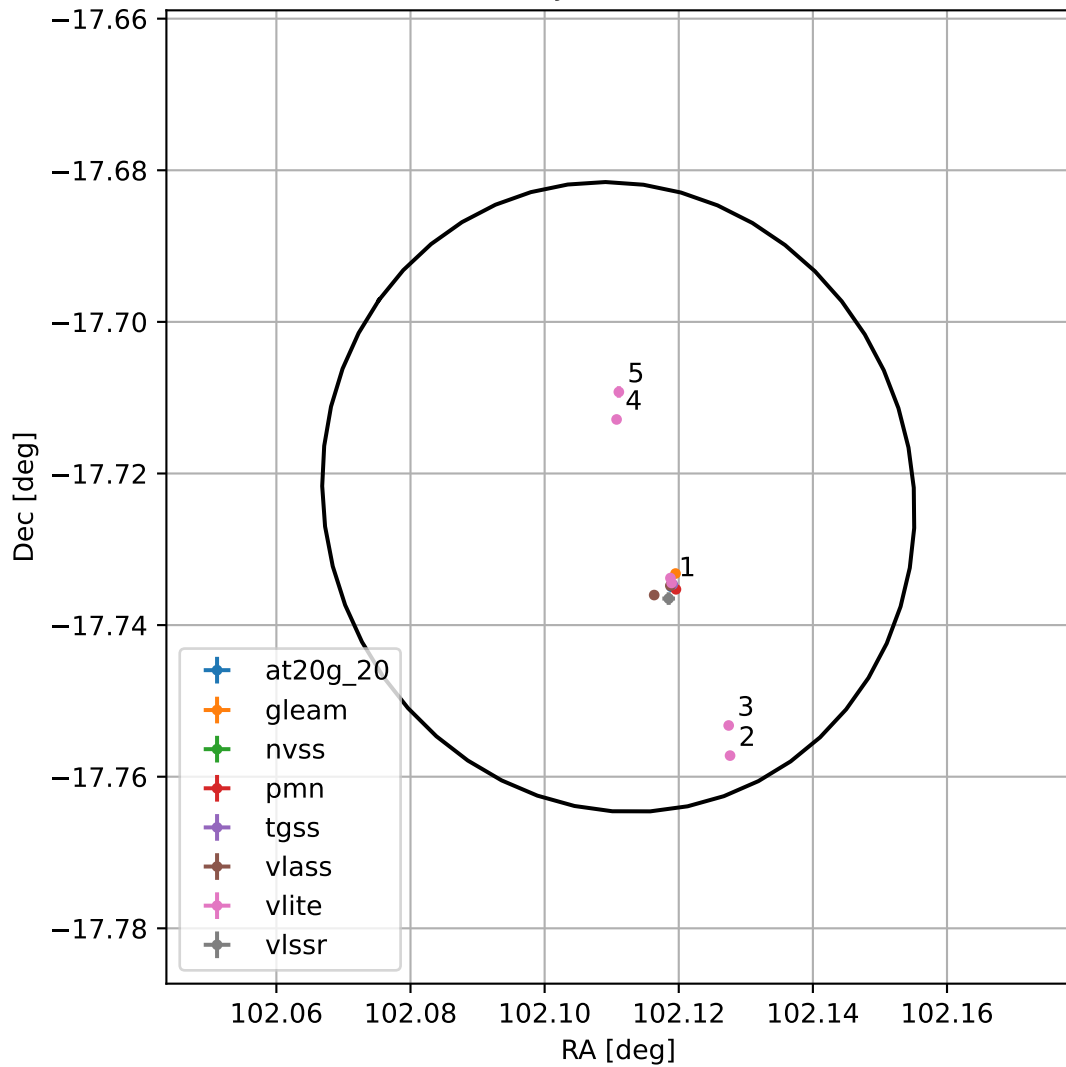
4FGL J0648.4-1743
