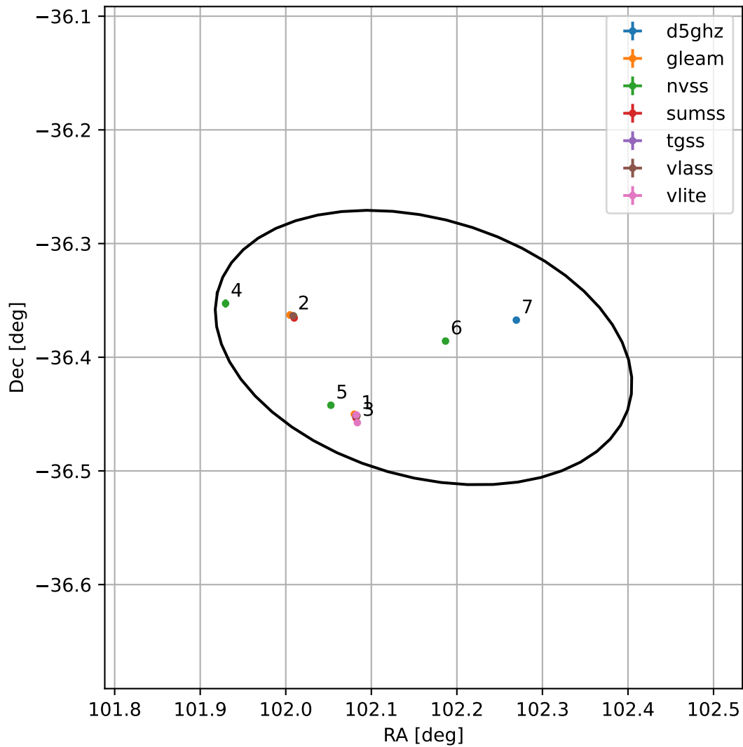
4FGL J0648.6-3623
