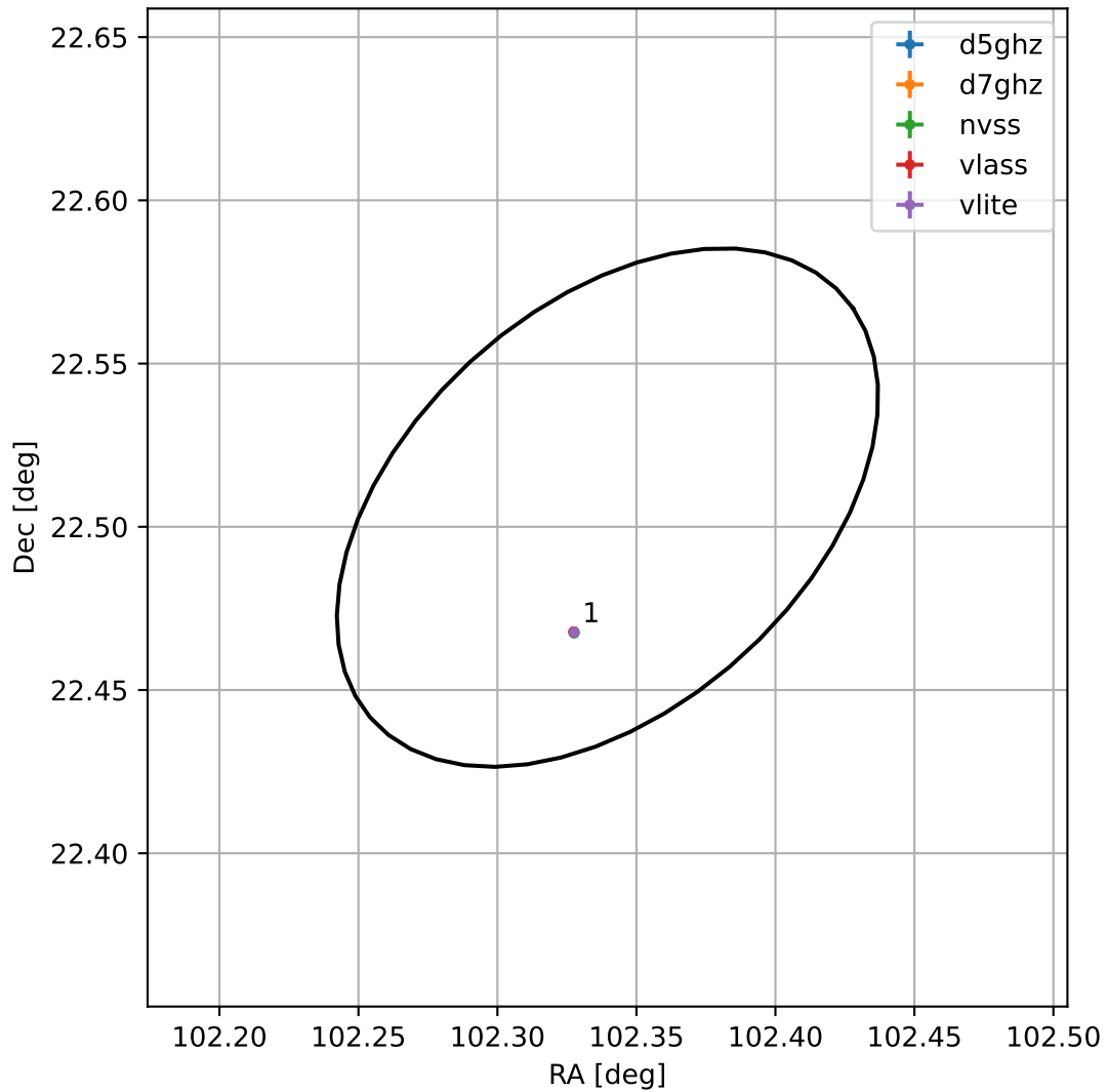
4FGL J0649.3+2230
