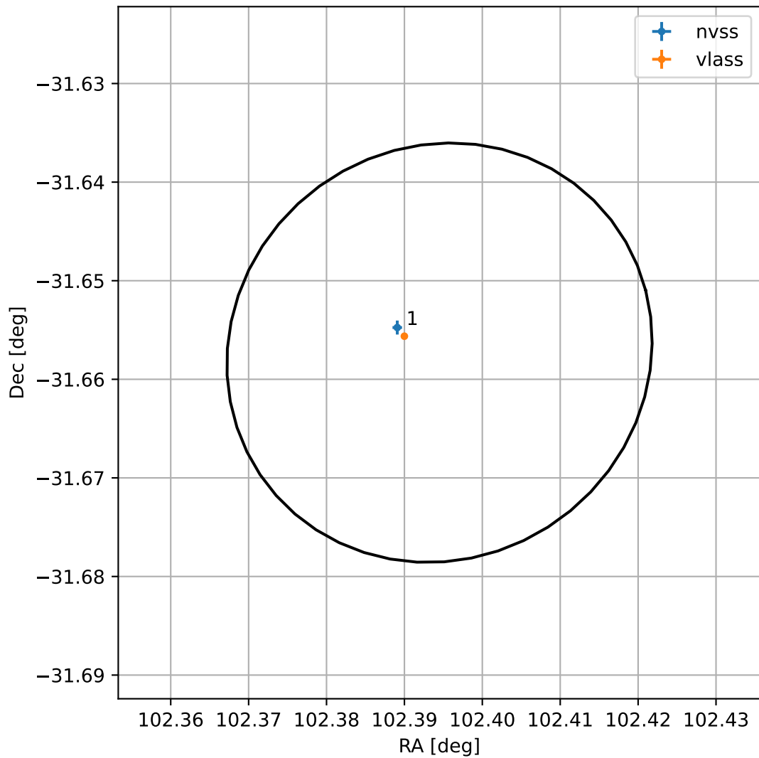
4FGL J0649.5-3139
