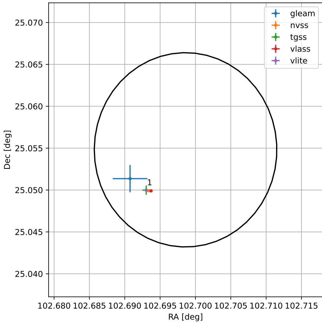
4FGL J0650.7+2503
