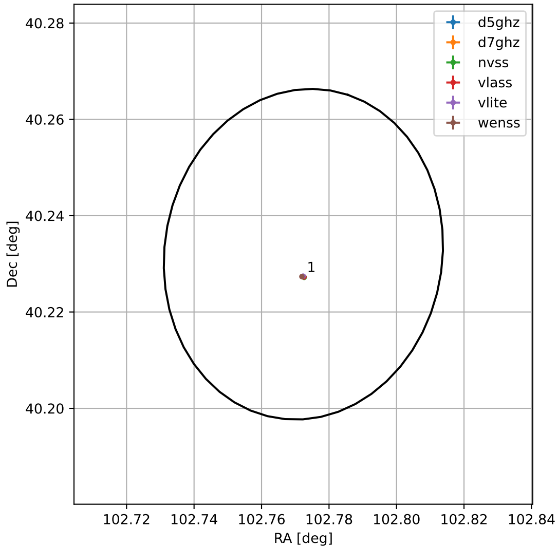
4FGL J0651.0+4013
