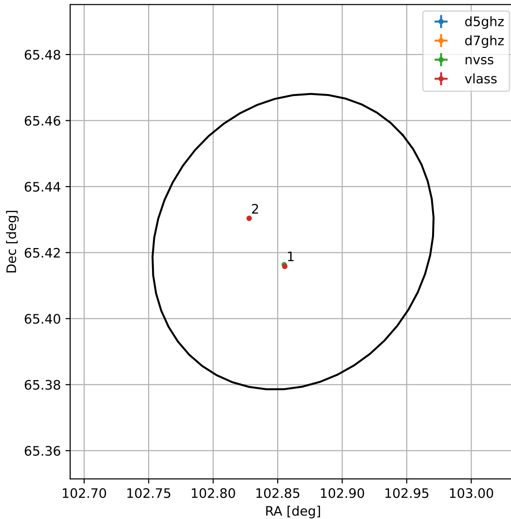
4FGL J0651.4+6525
