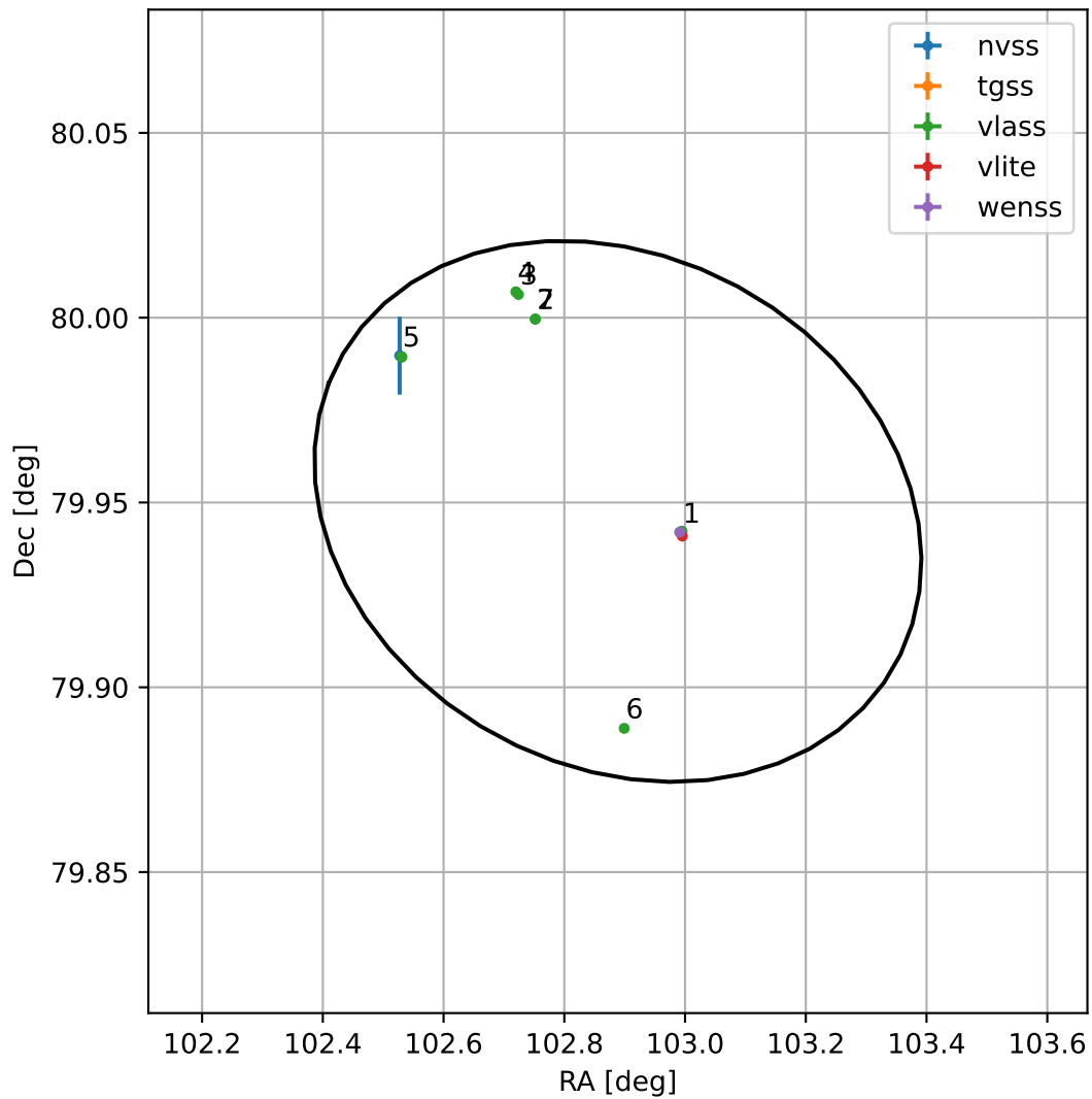
4FGL J0651.5+7956
