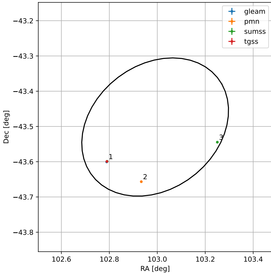
4FGL J0651.9-4330
