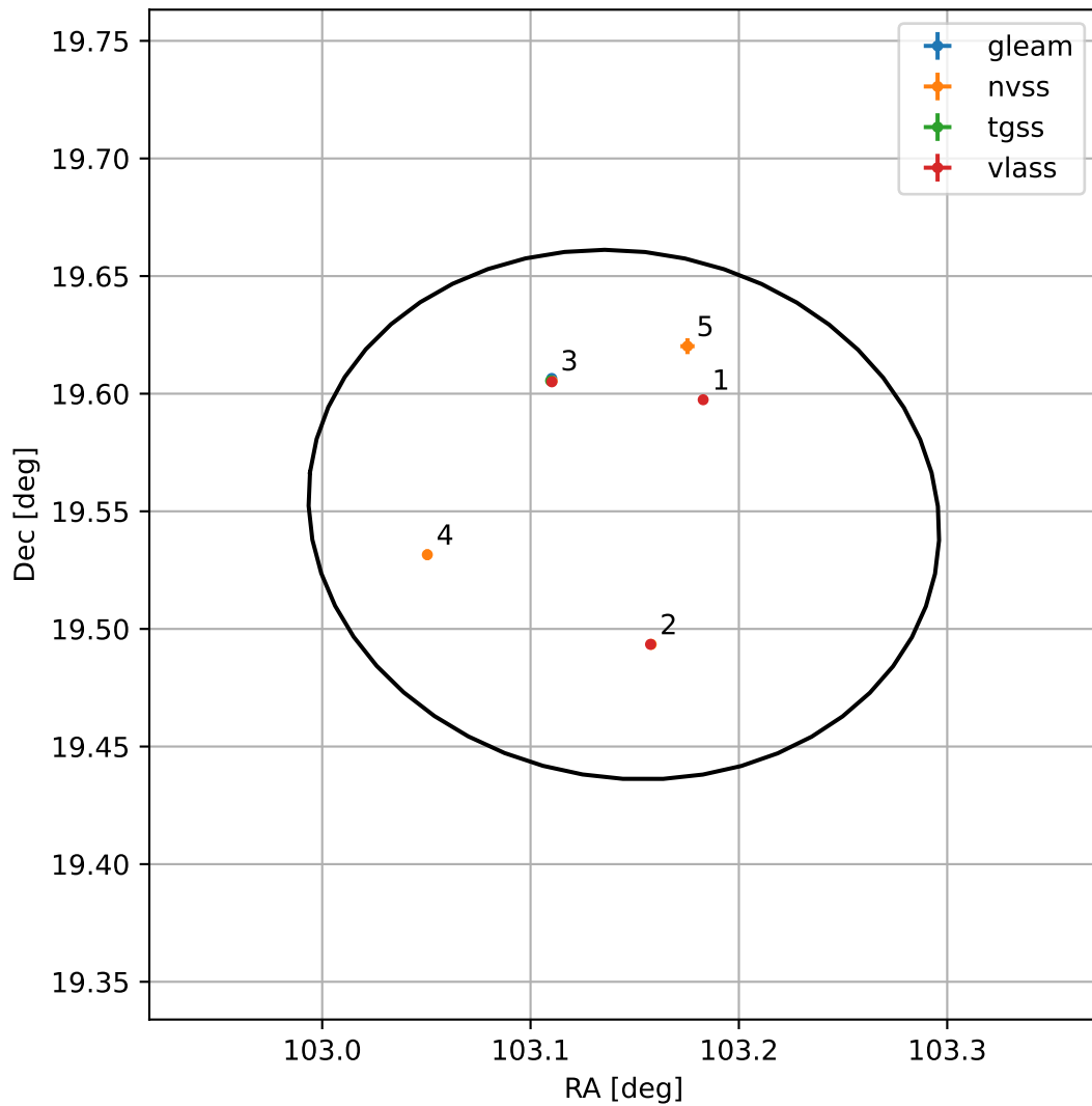
4FGL J0652.5+1932
