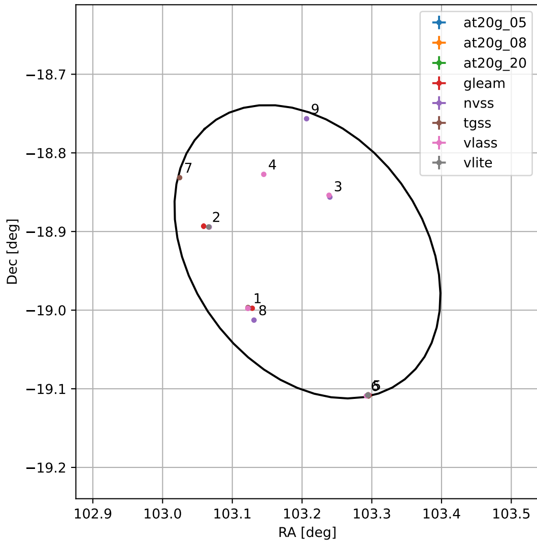
4FGL J0652.8-1855
