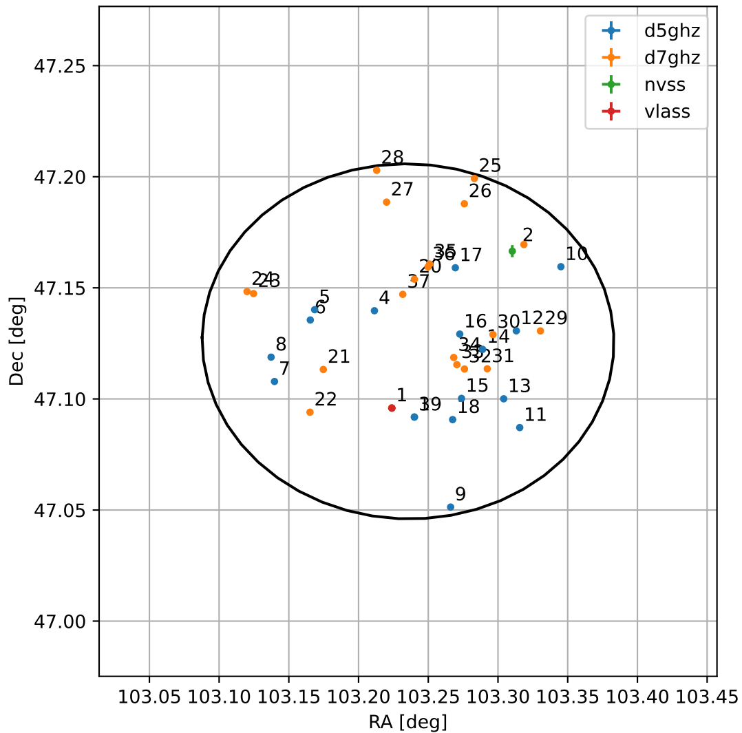
4FGL J0652.9+4707
