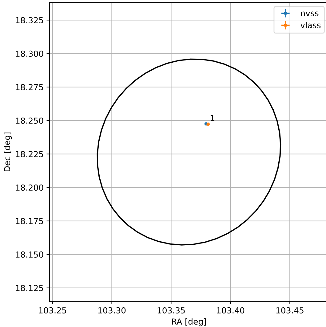
4FGL J0653.4+1813
