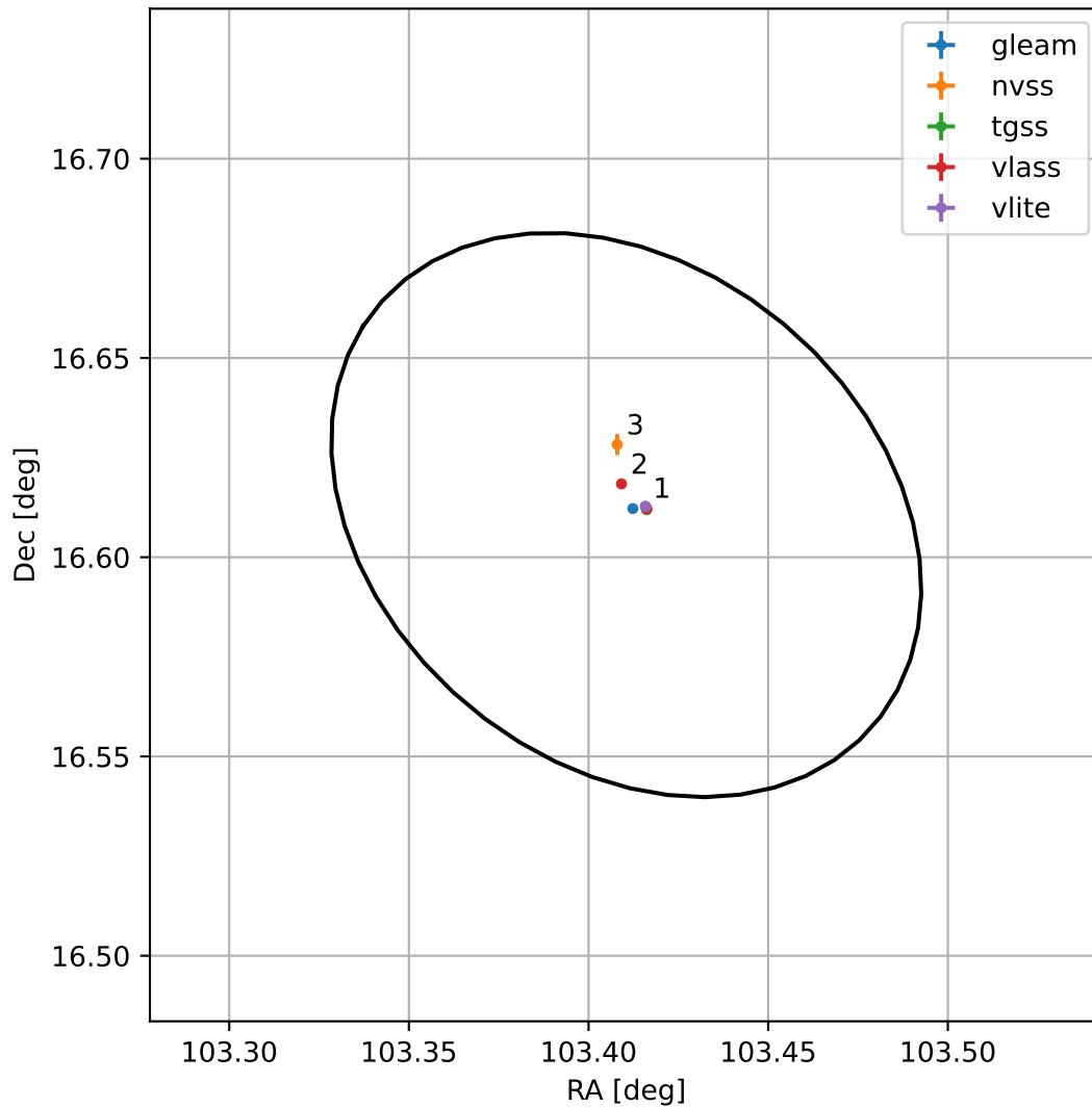
4FGL J0653.6+1636
