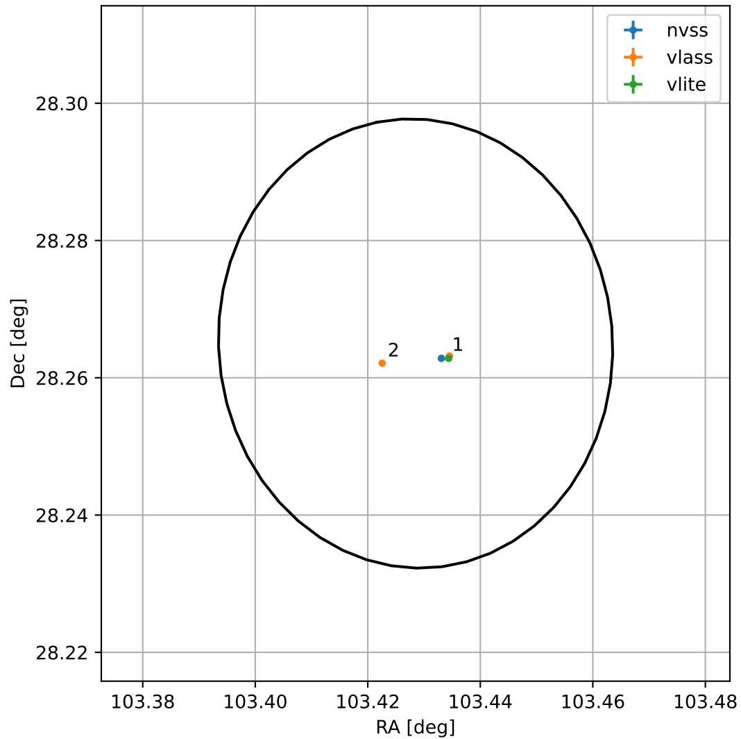
4FGL J0653.7+2815
