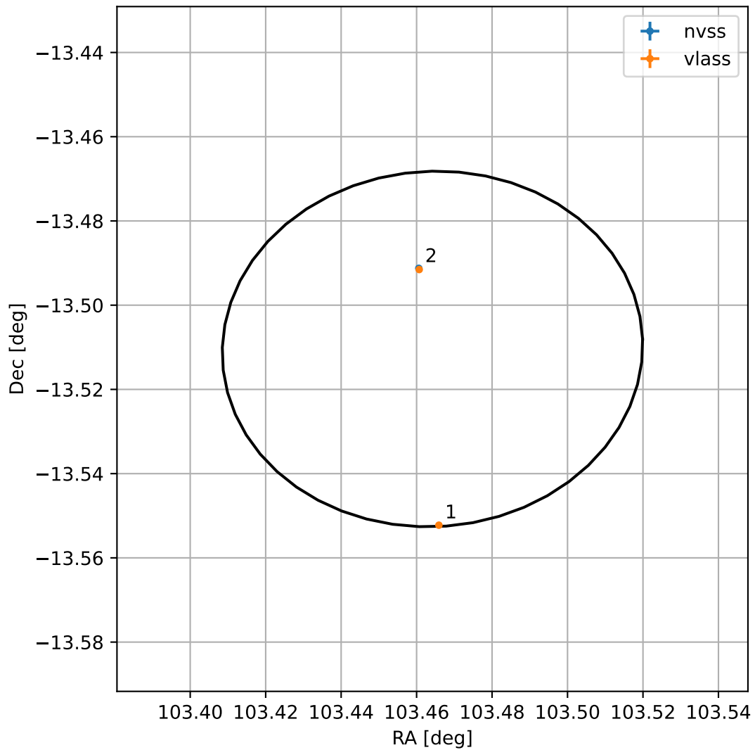
4FGL J0653.8-1330
