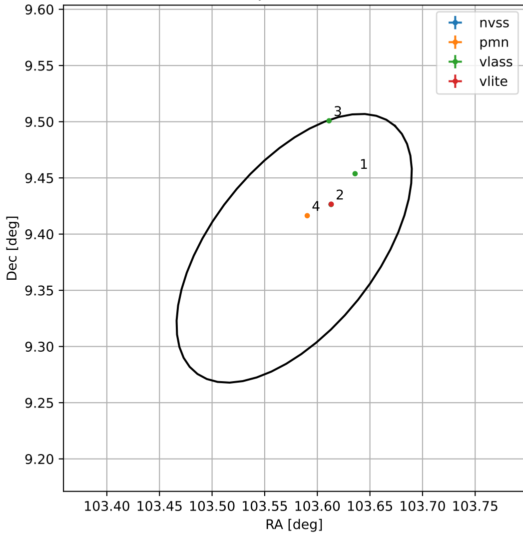
4FGL J0654.3+0923
