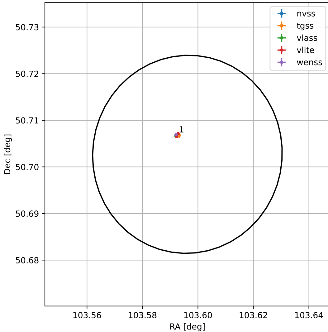
4FGL J0654.3+5042
