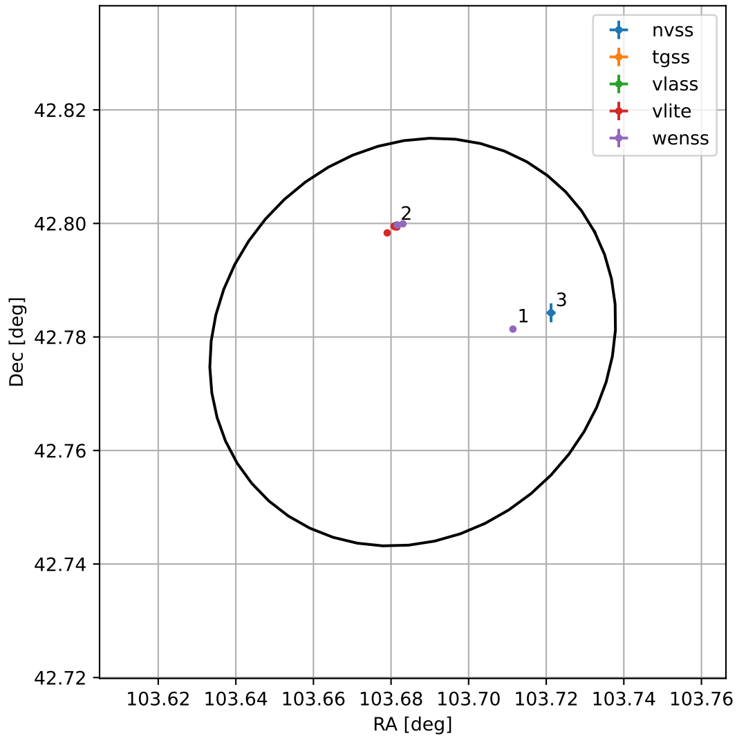
4FGL J0654.7+4246
