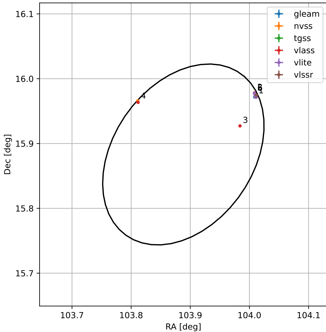
4FGL J0655.5+1552
