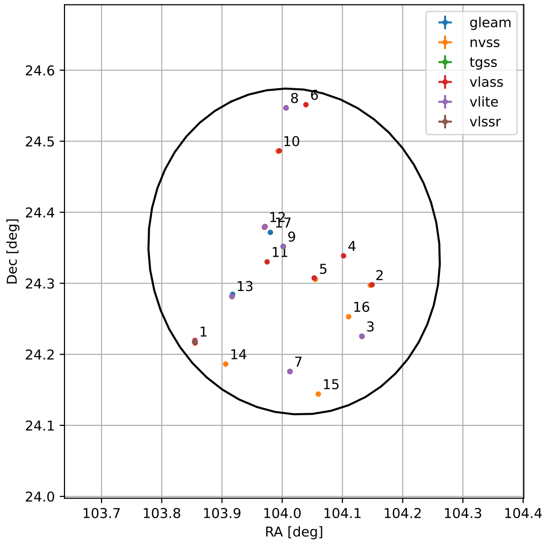
4FGL J0656.0+2420
