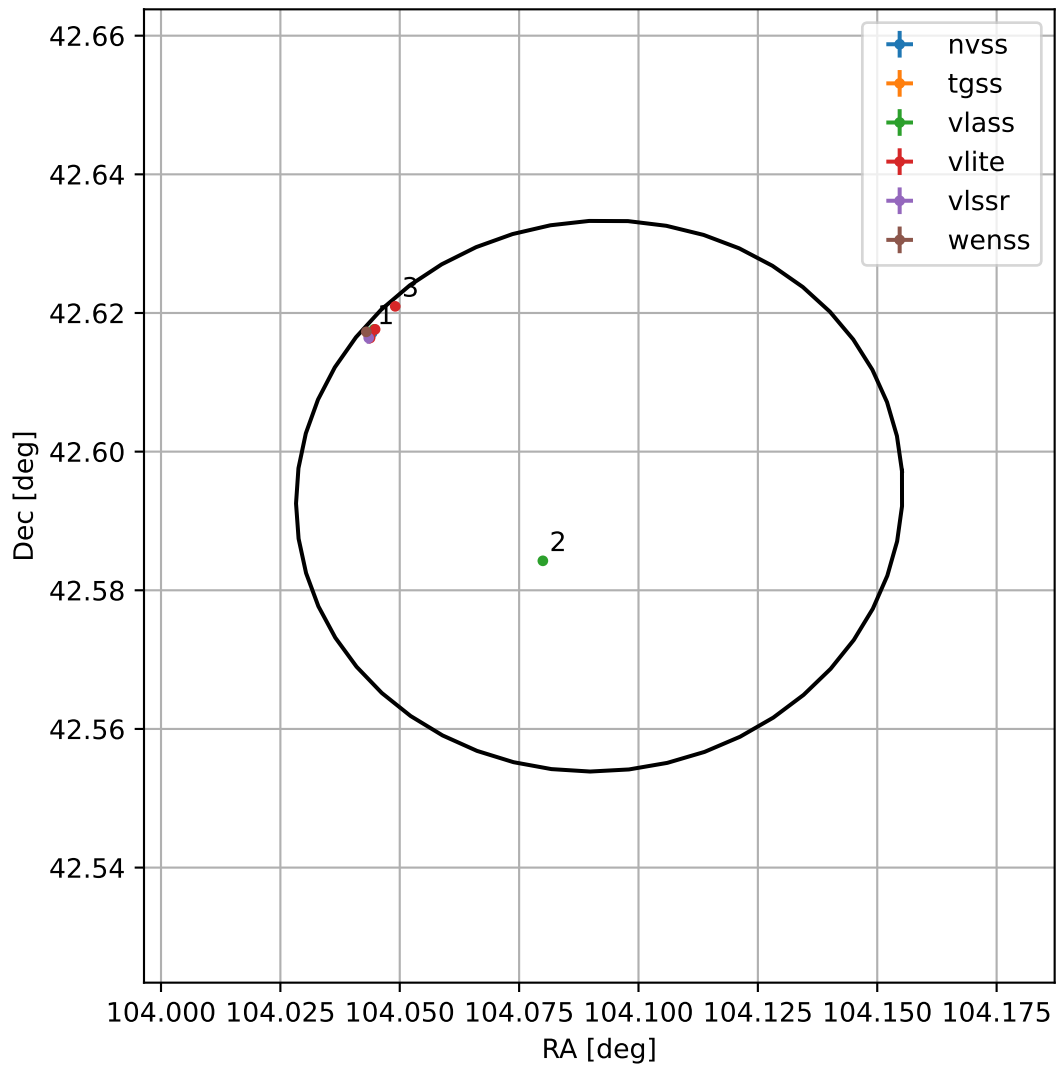
4FGL J0656.3+4235
