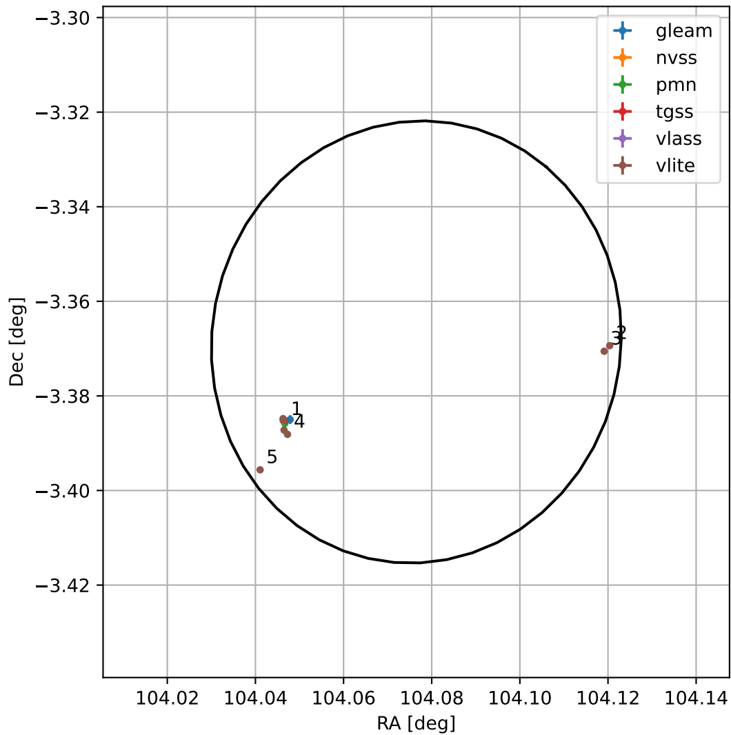
4FGL J0656.3-0322
