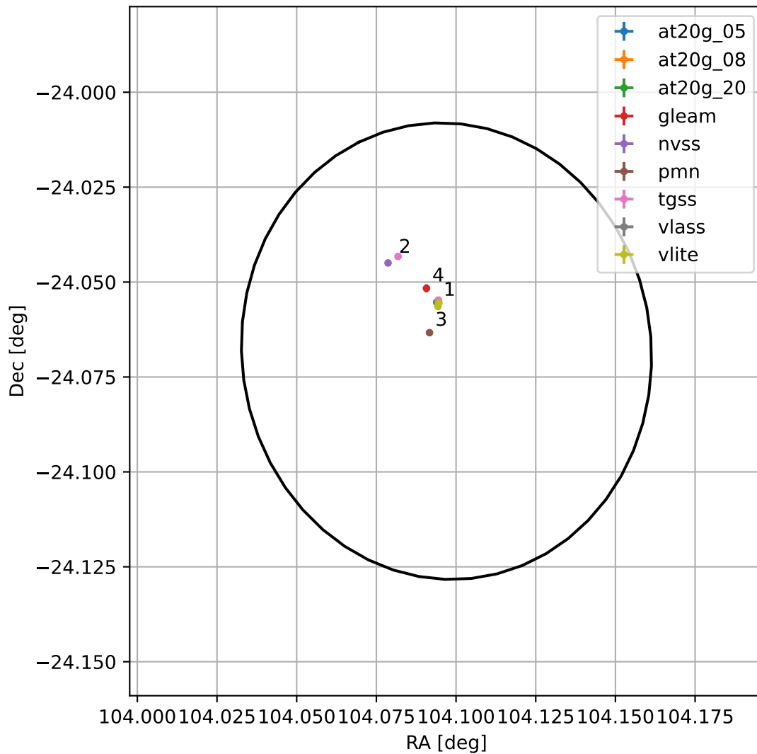
4FGL J0656.3-2404
