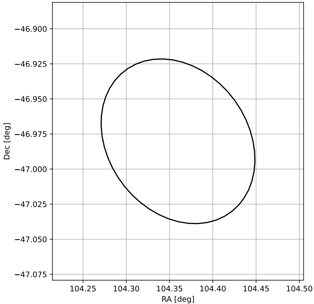
4FGL J0657.4-4658
