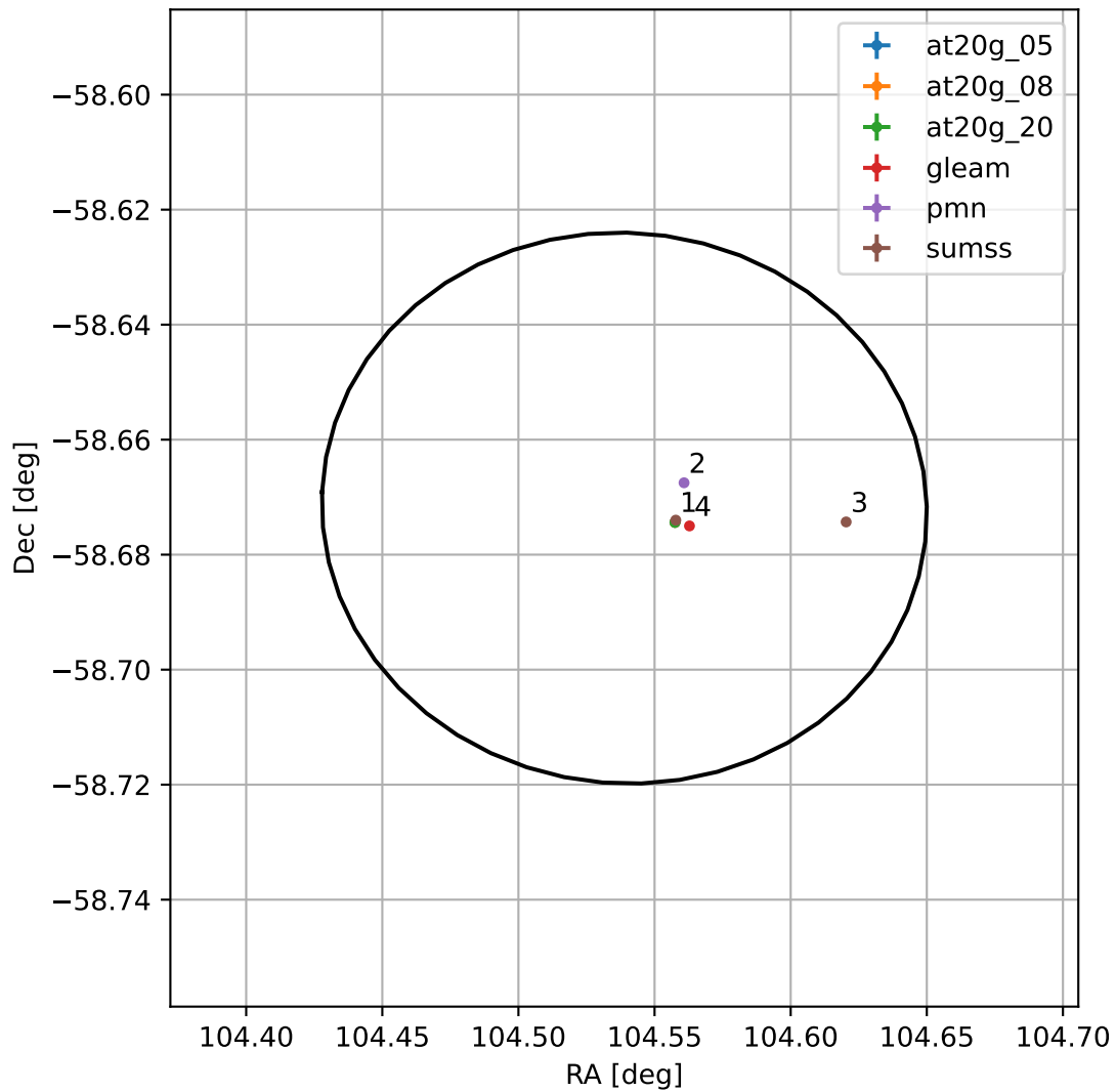
4FGL J0658.1-5840
