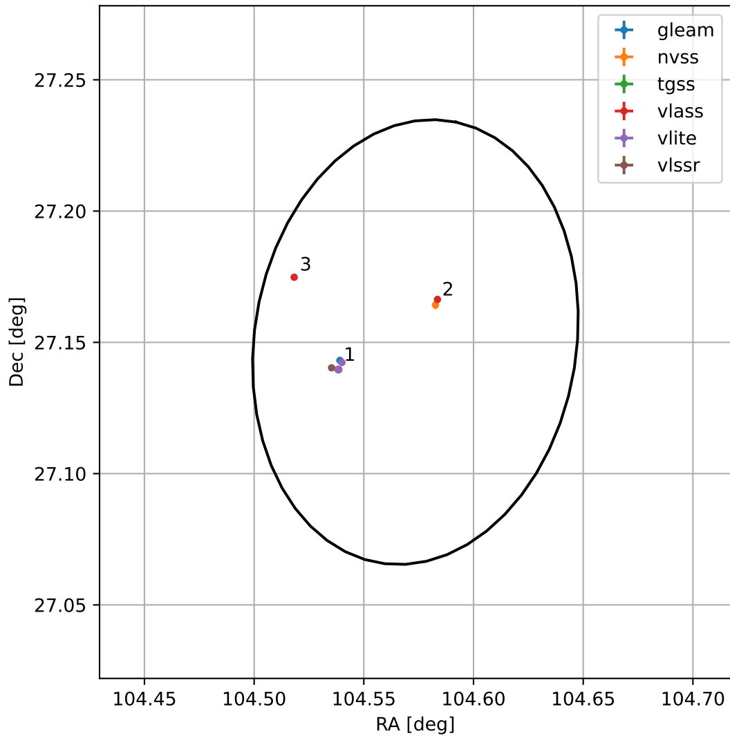
4FGL J0658.2+2709
