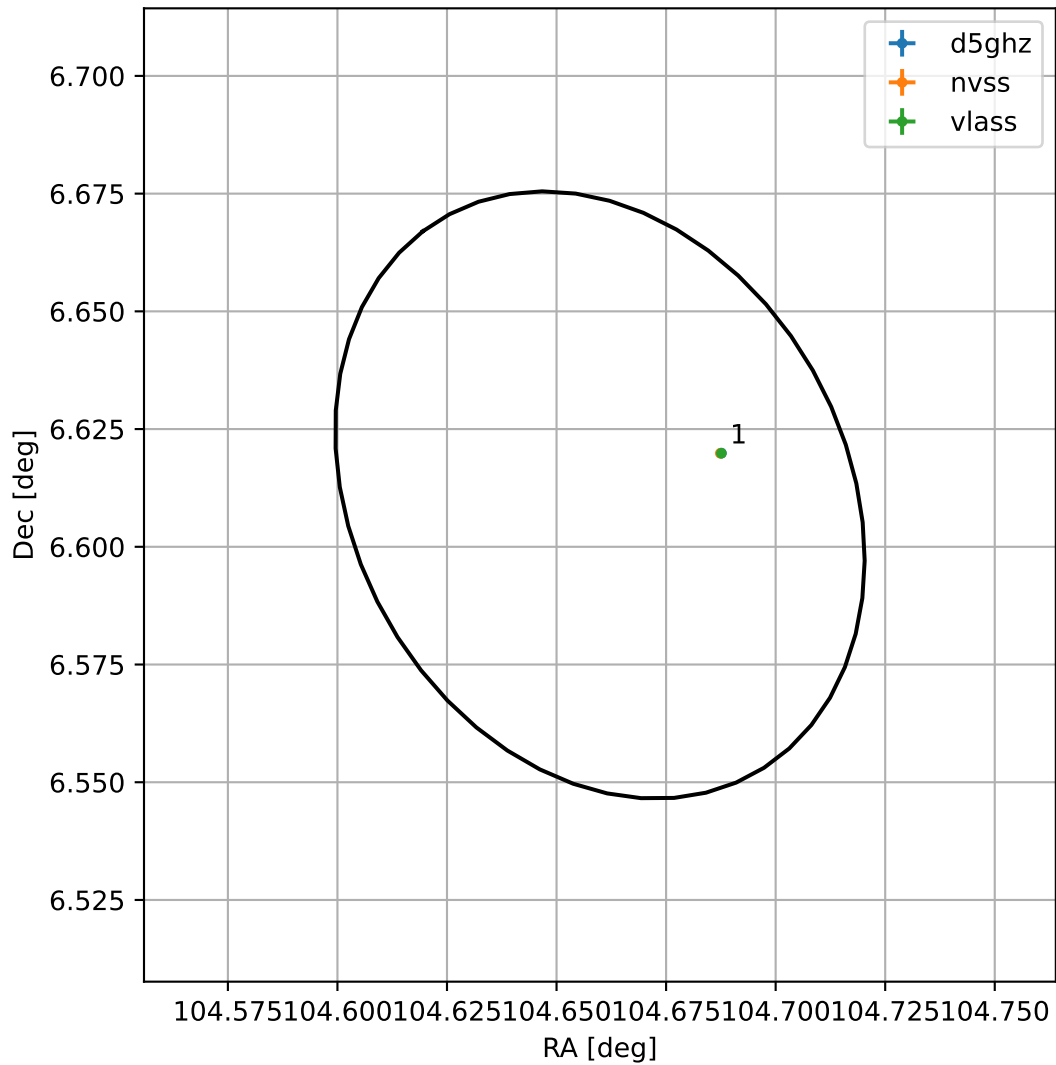
4FGL J0658.6+0636
