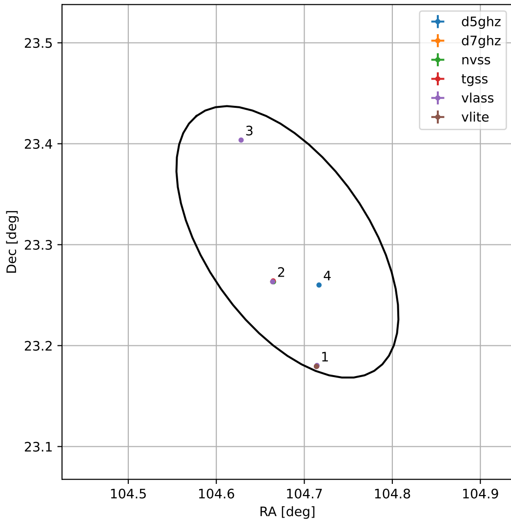
4FGL J0658.7+2318
