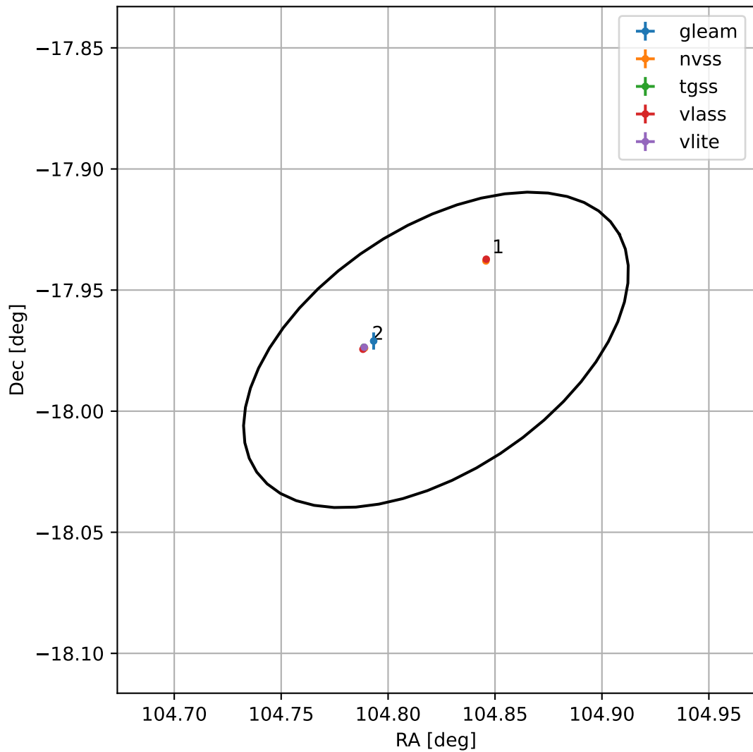
4FGL J0659.2-1758
