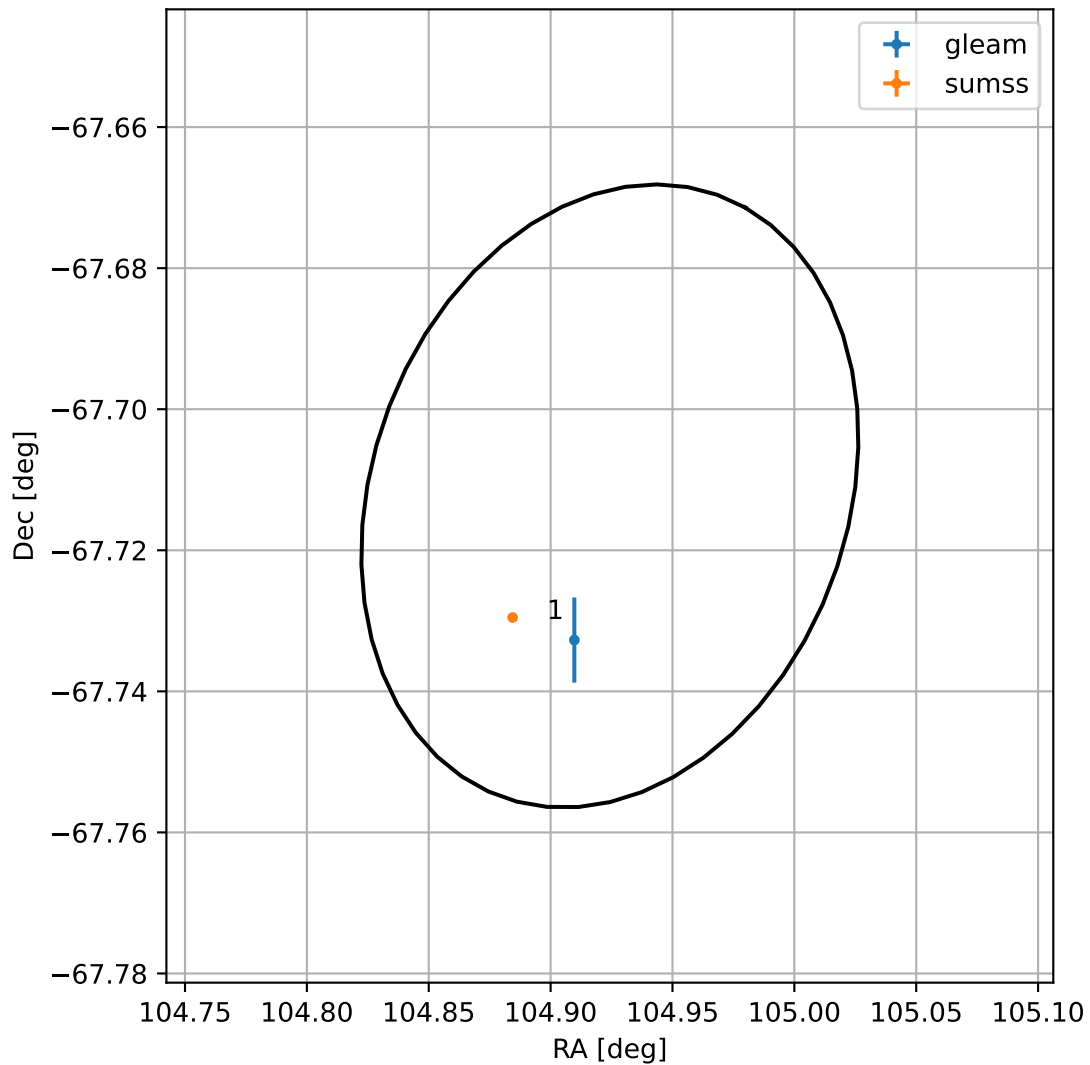
4FGL J0659.6-6742
