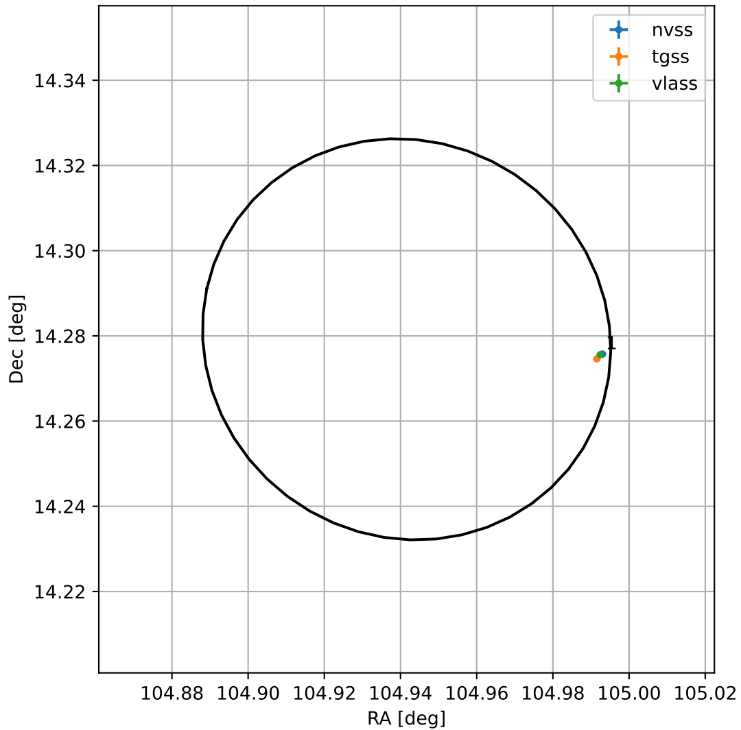
4FGL J0659.7+1416
