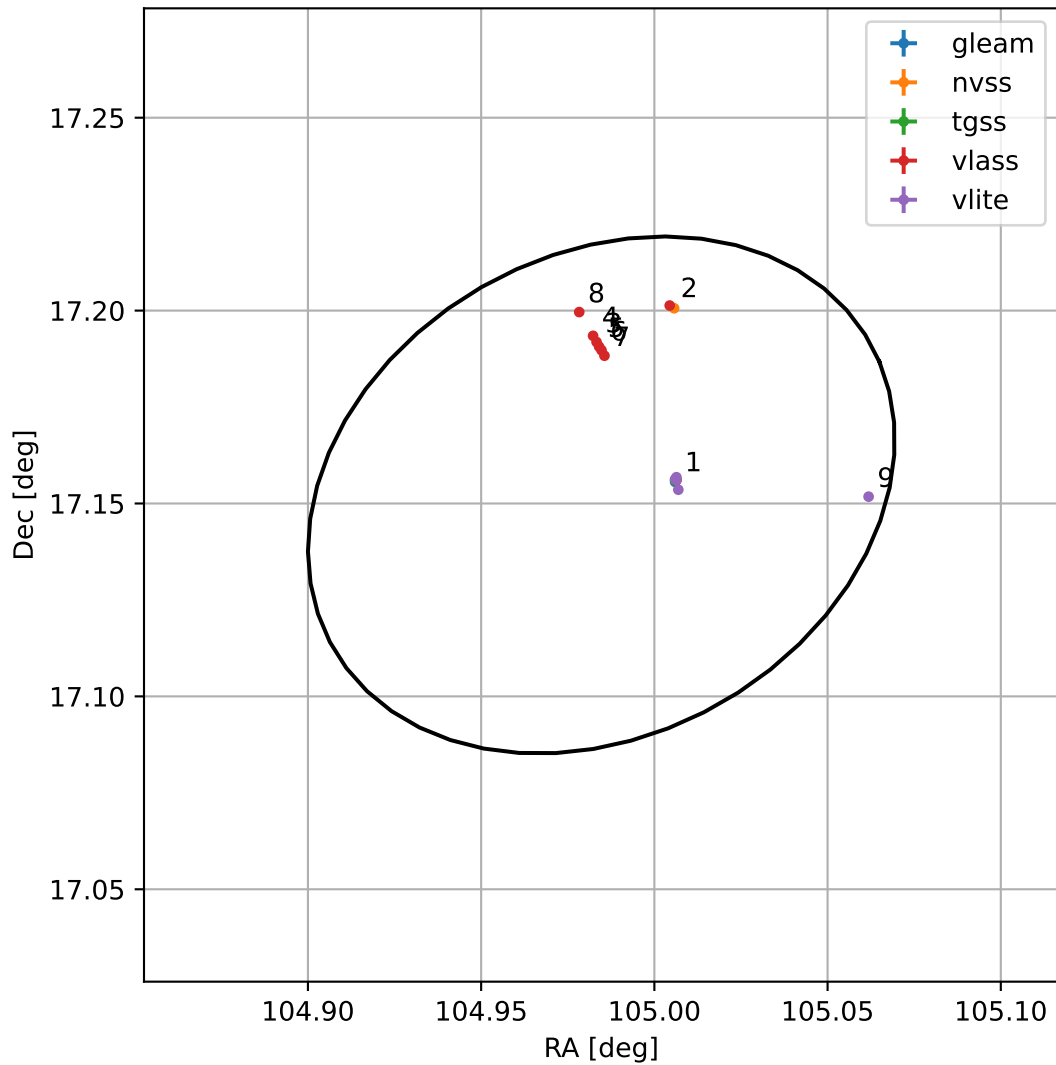
4FGL J0659.9+1709
