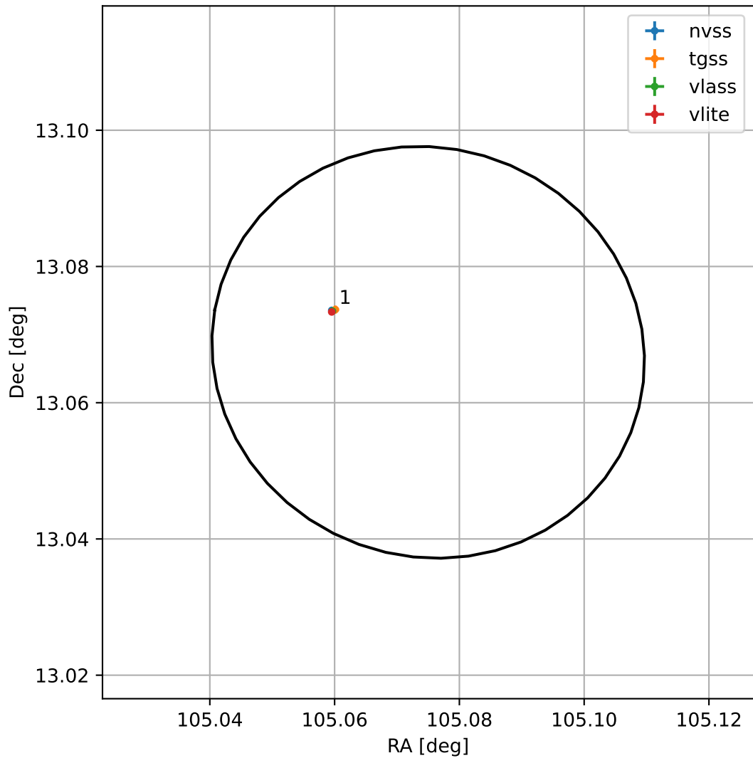
4FGL J0700.2+1304
