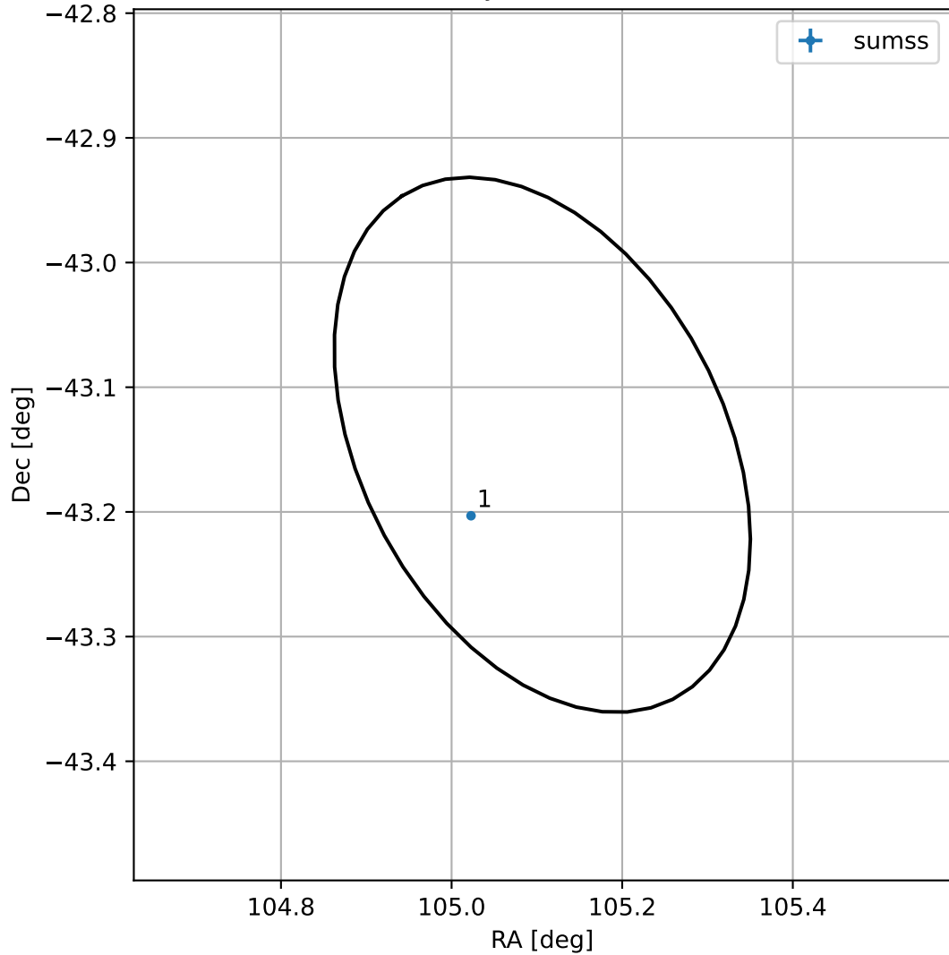
4FGL J0700.4-4308
