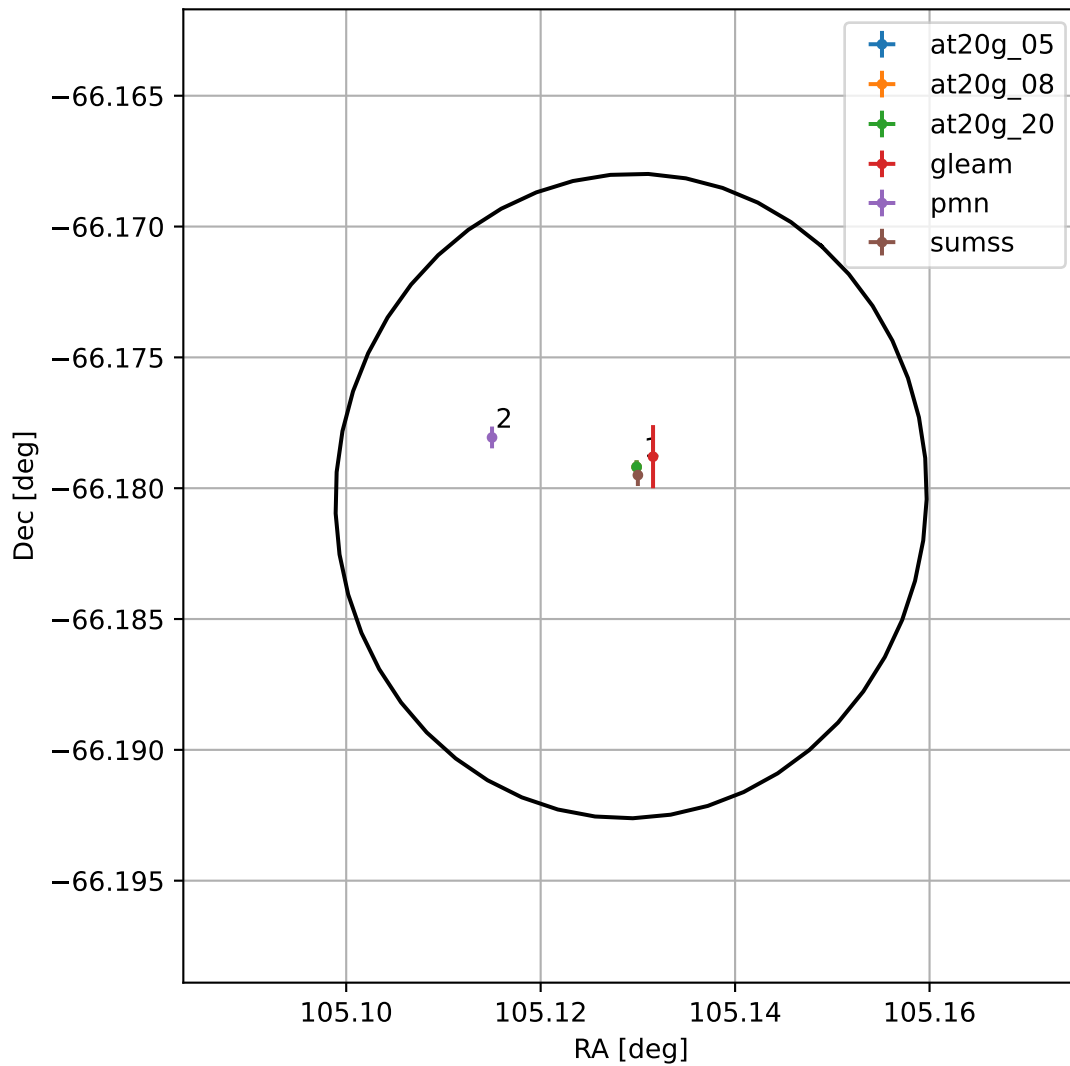
4FGL J0700.5-6610
