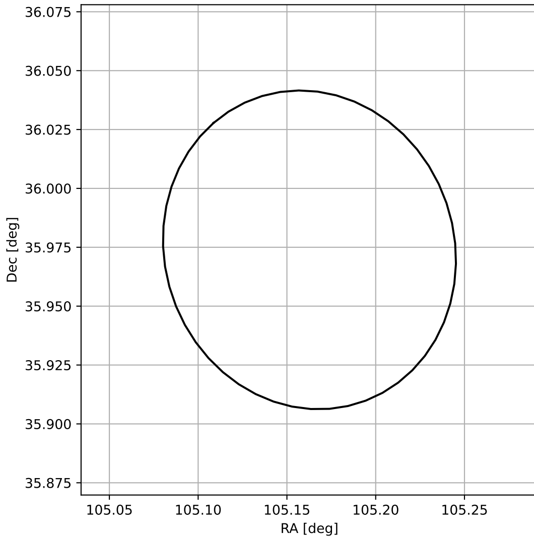
4FGL J0700.6+3558
