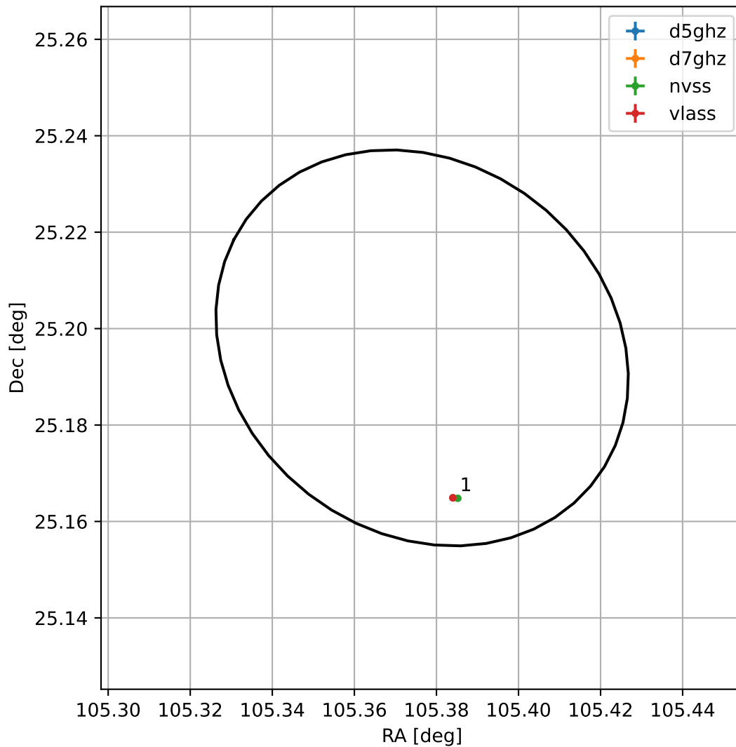
4FGL J0701.5+2511
